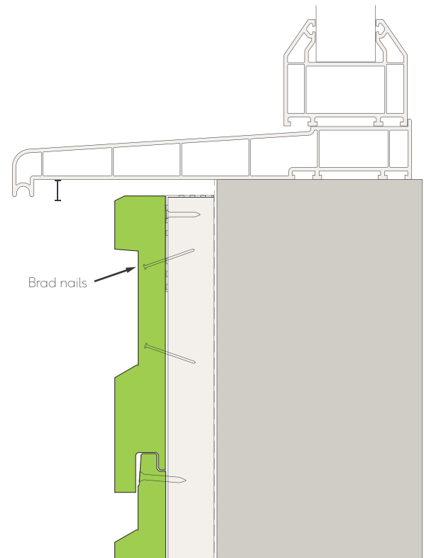
Fig. 16 - Window/door sill junction detail - brad nails
