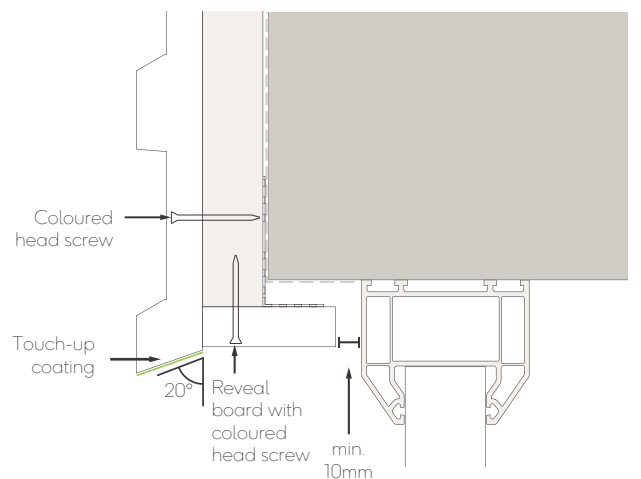
Fig. 13 - Window/door head with angled cut
