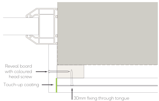
Fig. 15 - Window/door jamb with reveal boards
