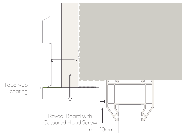
Fig. 14 - Window/door head with reveal boards
