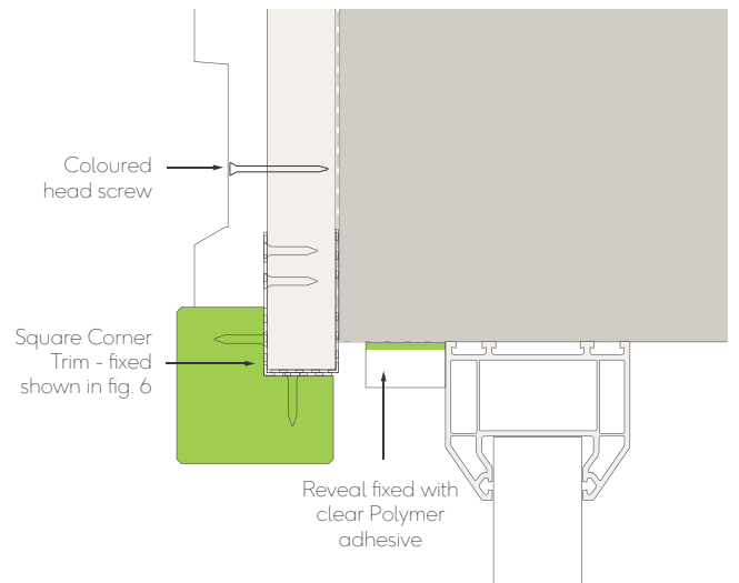
Fig. 12 - Window/door head with corner trim
