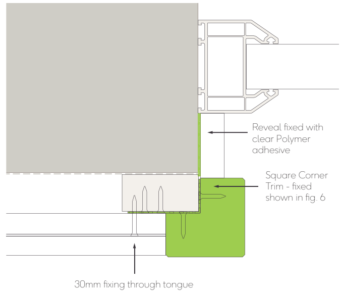
Fig. 11 - Window/door jamb with corner trim
