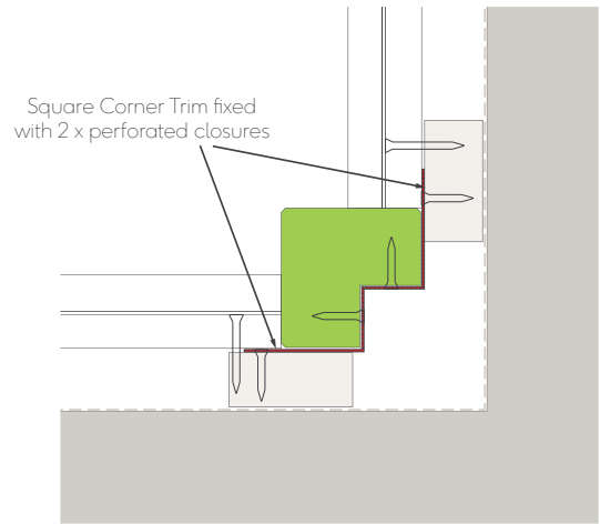
Fig. 7 - Internal corner detail
